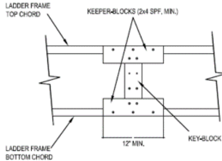
Detail 1.2
