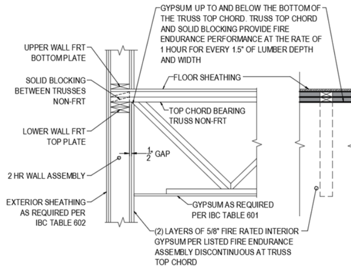
FIGURE 1. TOP CHORD BEARING TRUSS INTERSECTING TYPE IIIA WALL ASSEMBLY IBC SECTION 715 CODE COMPLIANT
