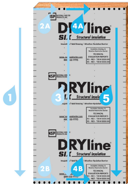
Figure 9. Installation, Step 3
