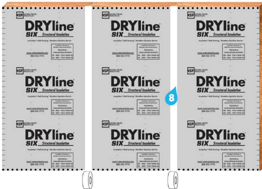
Figure 11. Installation, Step 5
