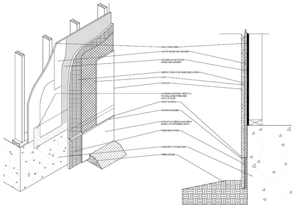
Figure 2. Stucco Veneer
