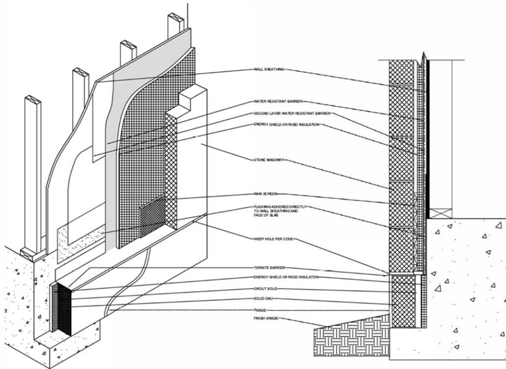
Figure 3. Stone Masonry Veneer
