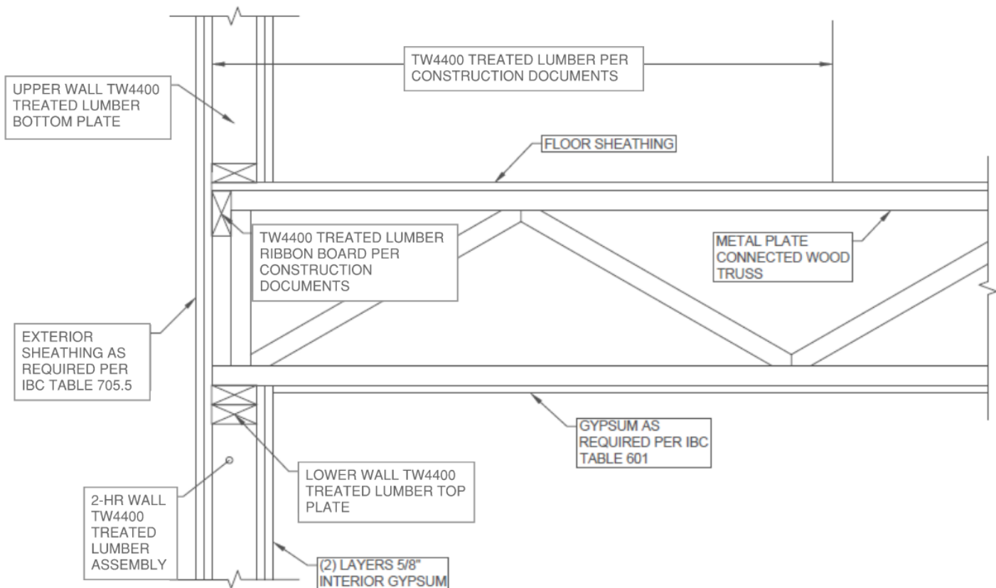
Figure 1. Truss End with Ribbon Board Detail for Type III Exterior Walls where Truss Ends are treated with TW4400.
