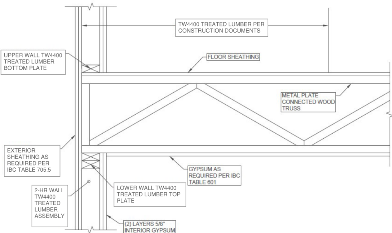
Figure 1. Truss End Detail for Type III Exterior Walls where Truss Ends are treated with TW4400.
