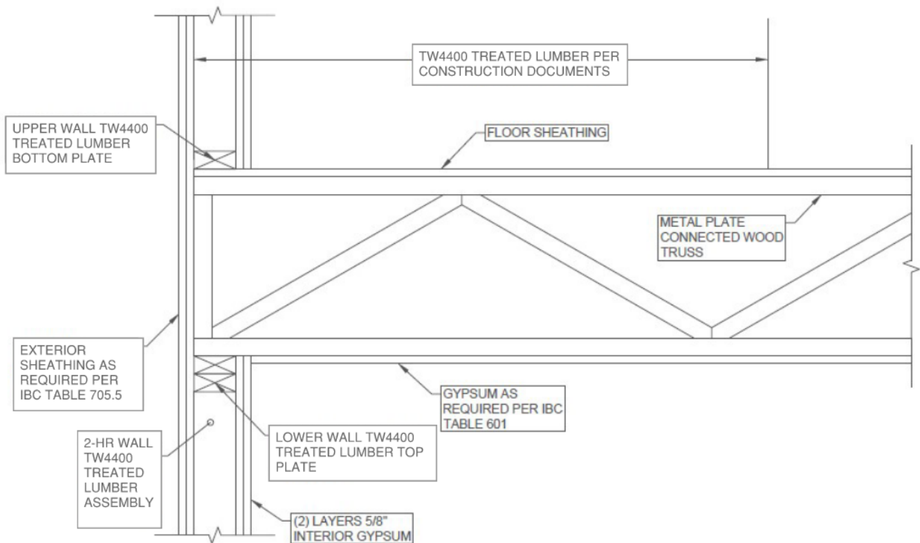
Figure 1. Truss End Detail for Type III Exterior Walls where Truss Ends are treated with TW4400
