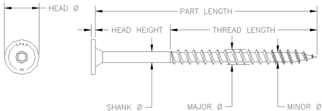
Figure 3. SPAX T-Star Pancake Head PowerLags Fastener
