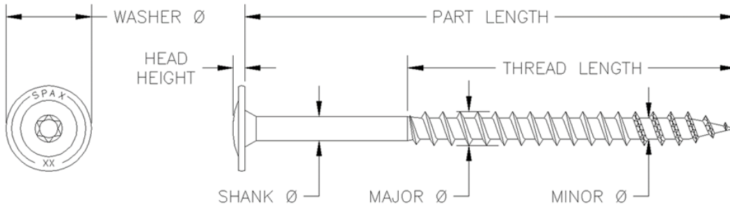
Figure 2. SPAX T-Star Washer Head PowerLags Fastener
