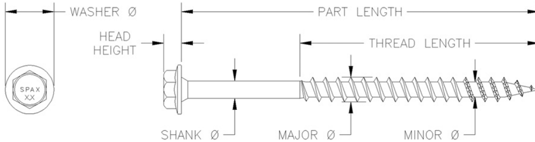
Figure 1. SPAX Hex Washer Head PowerLags Fastener
