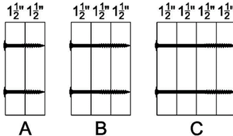
Figure 2. SPAX 5/16" T-Star Washer Head PowerLag Fasteners Assemblies for Truss and Sawn Lumber
